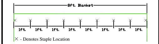
Figure E - Plan View
