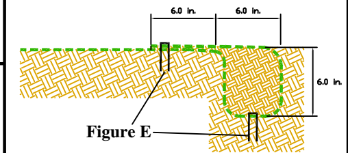
Figure E - Profile View
