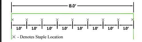
Figure E - Plan View
